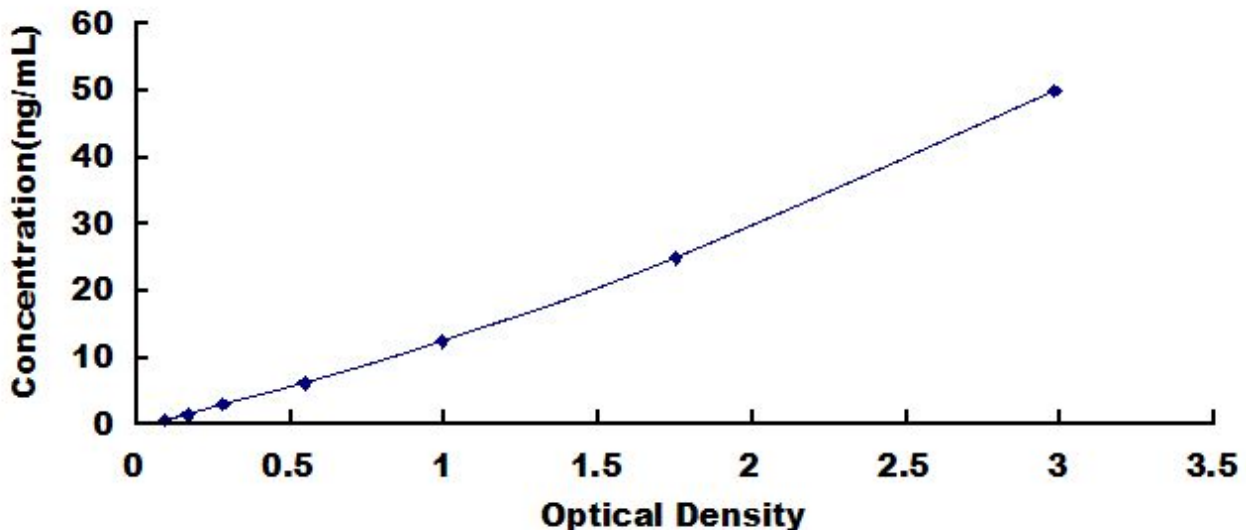
Typical Standard Curve for CAMP, Mouse ELISA.
